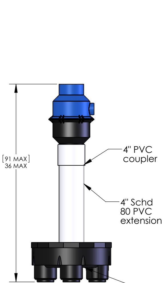
DETAIL Optional Extension SCALE 1 : 10
