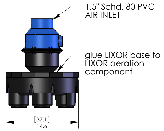
DETAIL 1 unit per blower SCALE 1 : 10
