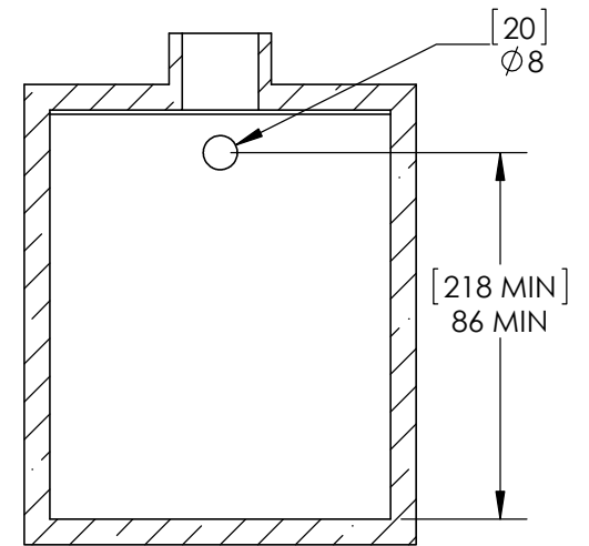
SECTION H-H SCALE 1 : 50
